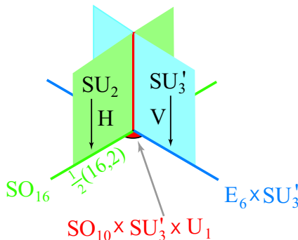
Figure 6: The neighborhood of one of the \alpha\beta\gamma -invariant four-plane intersections inside the lower end-of-the-world. Indicated in this diagram are the E_8 subgroups \mathcal{G}_\alpha = SO_{16} and \mathcal{G}_\gamma = E_6 \times SU_3 which survive on the \alpha\beta -invariant six-plane (the green line) and the \beta\gamma -invariant six-plane (the blue line), respectively. Also indicated is the representation of the six-dimensional twisted hypermultiplet needed to cure six-dimensional anomalies locally on the \beta\gamma -plane.
