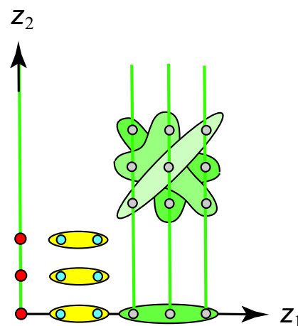
Figure 1: Points of the four-torus (z_1, z_2) identified by the \mathbb{Z}_2 \times \mathbb{Z}_3 subgroup of \Gamma generated by \alpha and \gamma . The red spots are the three \mathbb{Z}_2 \times \mathbb{Z}_3 invariant points, the yellow blobs are the \mathbb{Z}_3 -invariant \mathbb{Z}_2 -doublets with components in blue. The green lines are the four \mathbb{Z}_2 invariants. The green blobs encircle those \mathbb{Z}_3 triplets which provide noteworthy identifications.
